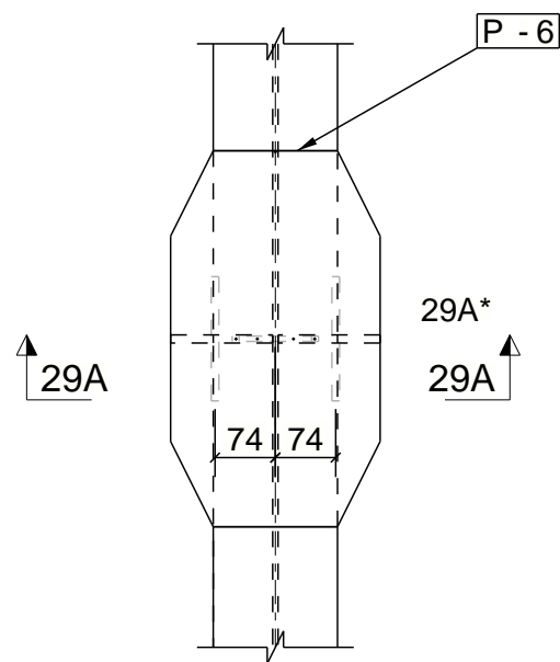
29 SHT. 02 DETAIL SCALE- 1:10 AS SHOWN AT 1 LOCATION
