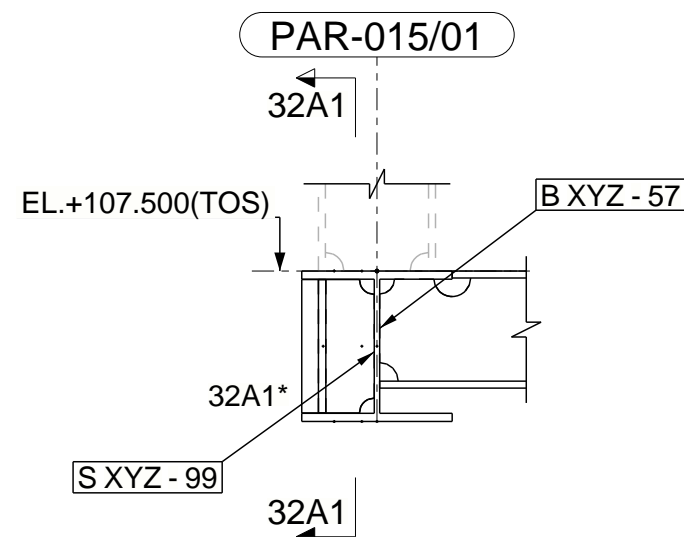
SECTION 32A - 32A SCALE - 1:10 32A * AS SHOWN AT 1 LOCATION
