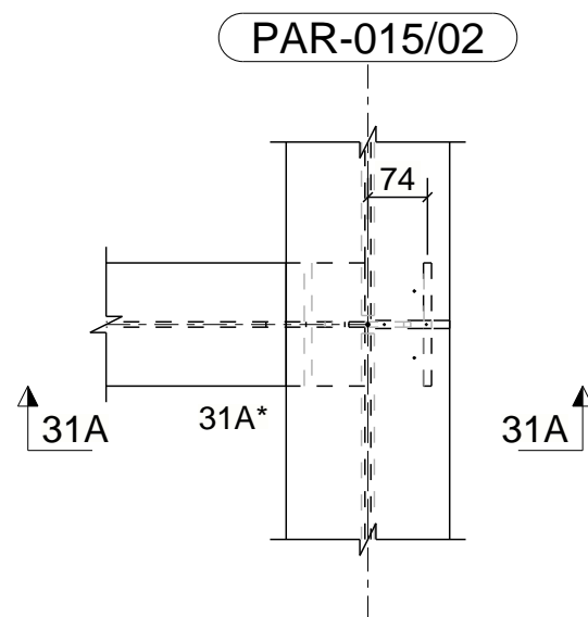
31 SHT. 02 DETAIL SCALE- 1:10 AS SHOWN AT 1 LOCATION
