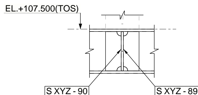
SECTION 30A1 - 30A1 SCALE - 1:10 30A1 * AS SHOWN AT 1 LOCATION
