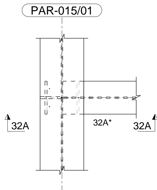
32 SHT. 02 DETAIL SCALE- 1:10 AS SHOWN AT 1 LOCATION
