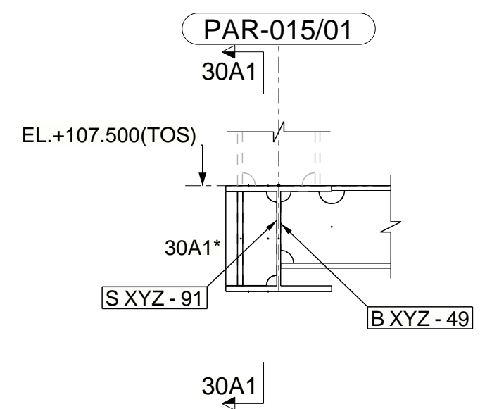
SECTION 30A - 30A SCALE - 1:10 30A * AS SHOWN AT 1 LOCATION
