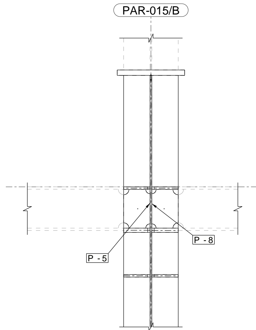
SECTION 3A - 3A SCALE - 1:10 3A * AS SHOWN AT 1 LOCATION
