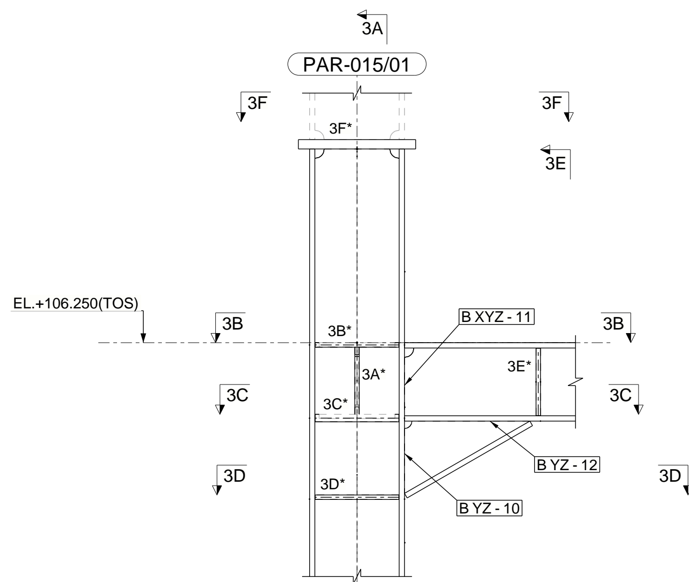
3 SHT. 01 DETAIL SCALE- 1:10 AS SHOWN AT 1 LOCATION
