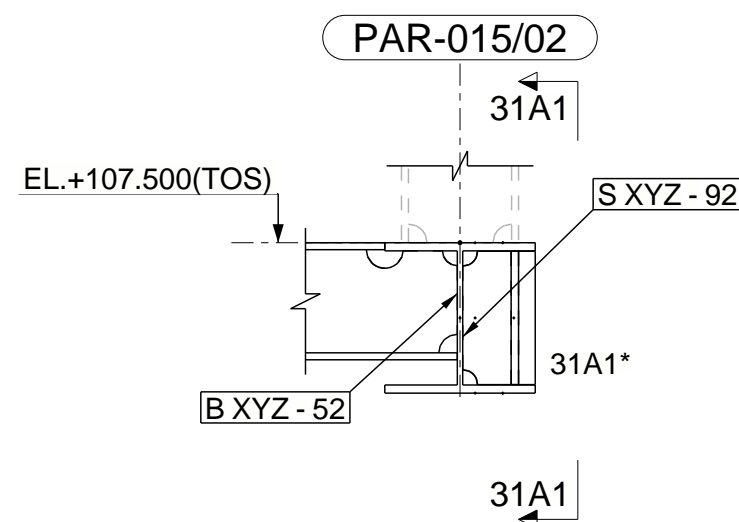
SECTION 31A - 31A SCALE - 1:10 31A * AS SHOWN AT 1 LOCATION
