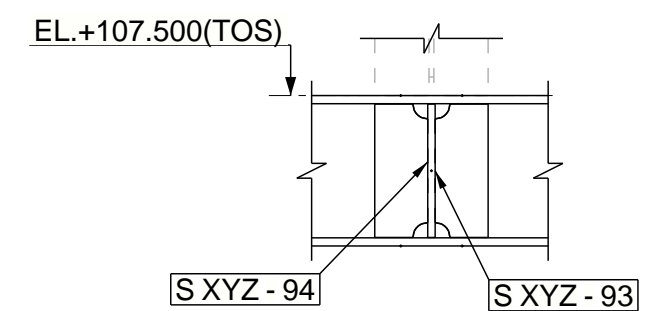
SECTION 31A1 - 31A1 SCALE - 1:10 31A1 * AS SHOWN AT 1 LOCATION
