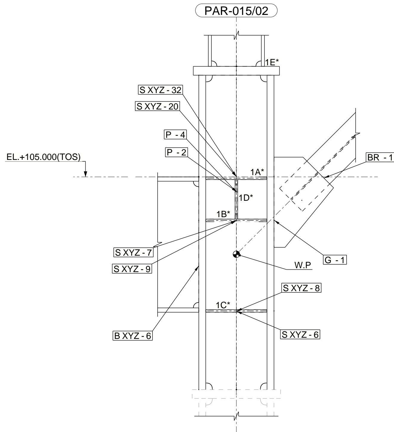
2 SHT. 01 DETAIL SCALE- 1:10 AS SHOWN AT 1 LOCATION
