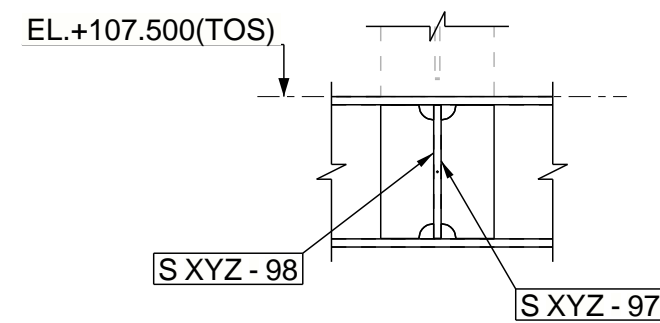
SECTION 32A1 - 32A1 SCALE - 1:10 32A1 * AS SHOWN AT 1 LOCATION
