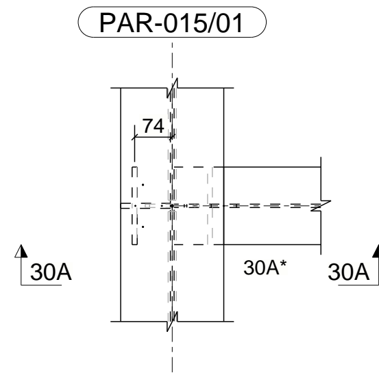
30 SHT. 02 DETAIL SCALE- 1:10 AS SHOWN AT 1 LOCATION
