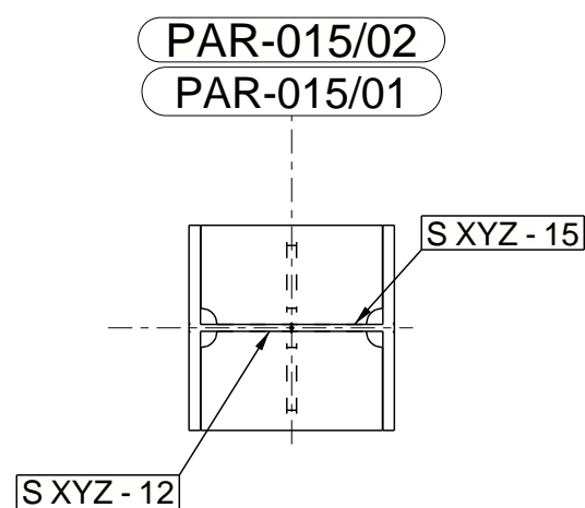
SECTION 3B - 3B SCALE - 1:10 3B * AS SHOWN AT 2 LOCATIONS
