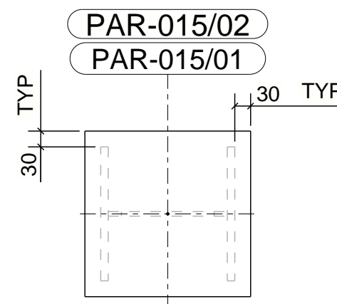
SECTION 3F - 3F SCALE - 1:10 3F * AS SHOWN AT 2 LOCATIONS
